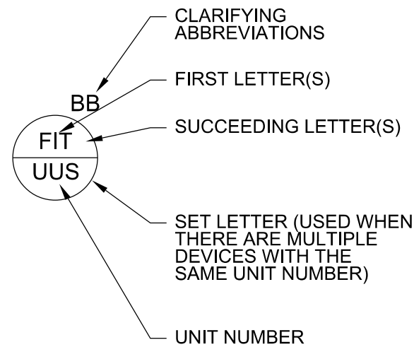
EXAMPLE P&ID SYMBOL
